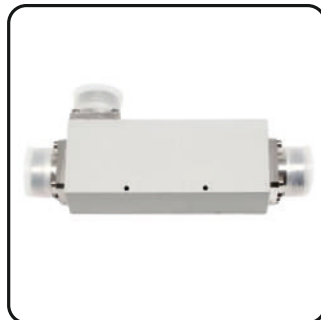
698 - 2700 MHz DIN Female 163 Pim 40 dB RF Directional Coupler
