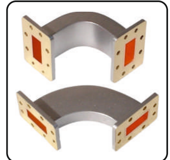
Waveguide Bend
