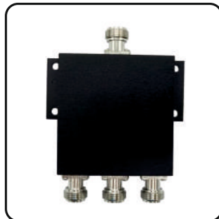
3 Way Power Splitter 150 ~ 1000 Mhz
