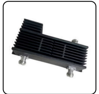
698 - 2700 MHz 4.3 - 10 Female 3 dB Hybrid Combiner Coupler
