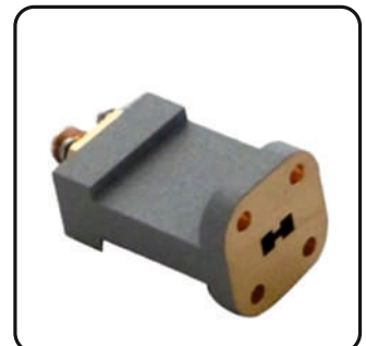
Double Ridge WG To Coaxial Adapter (End Launch)
