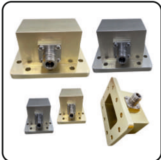
Waveguide To Coaxial Adapter RA
