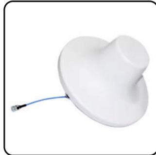
380-600 MHz Low Pim Indoor Omni Antenna
