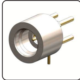
SMP Male R/A PCB Mount (4 LEG, R/A CONTACT)
